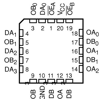
CY54FCT244T . . . L PACKAGE (TOP VIEW)
